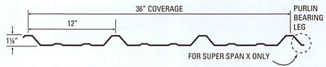
SUPER SPAN / SUPER SPAN X
