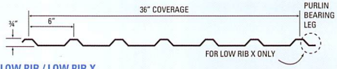
LOW RIB / LOW RIB X
